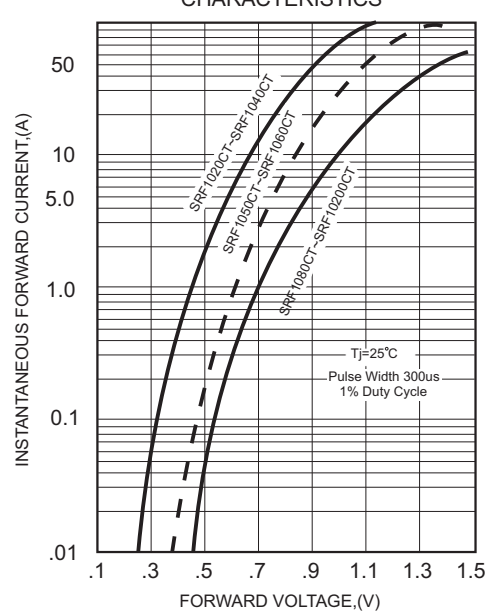
FIG.2-TYPICAL FORWARD CHARACTERISTICS
